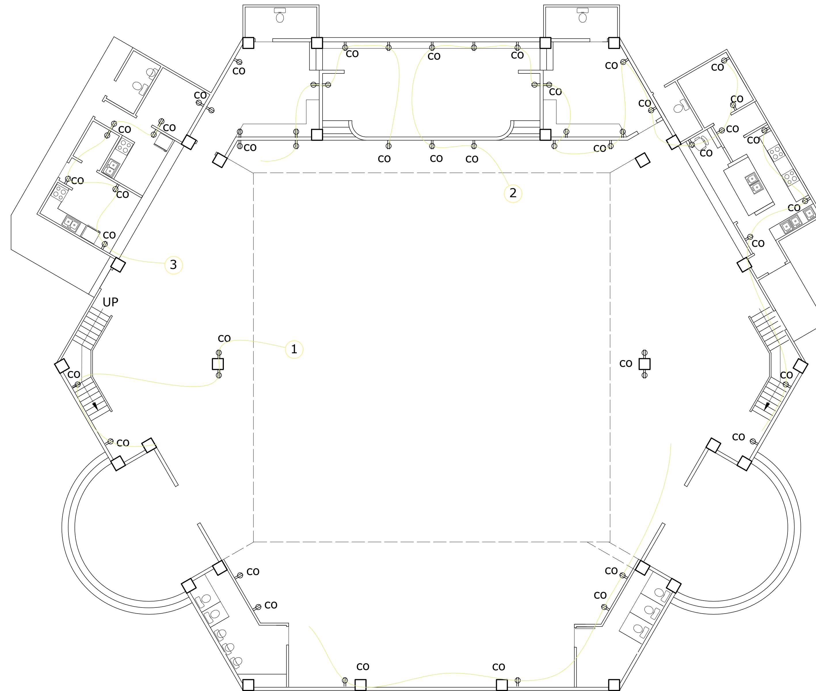
1 EL 01 SCALE 1: 100 MTS. GROUND FLOOR POWER LAYOUT
