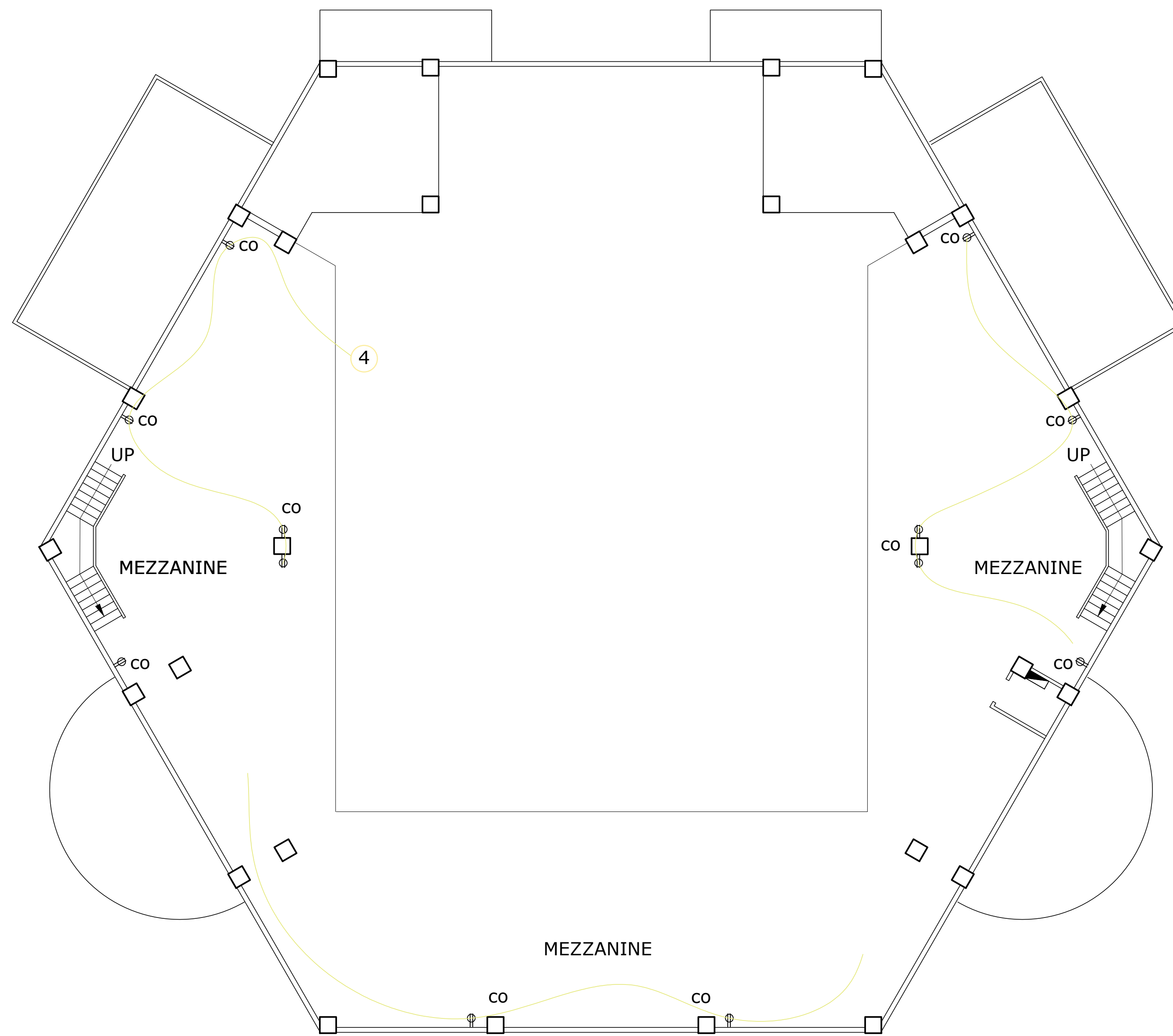
1 MEZZANINE POWER LAYOUT EL 02 SCALE 1: 100 MTS.
