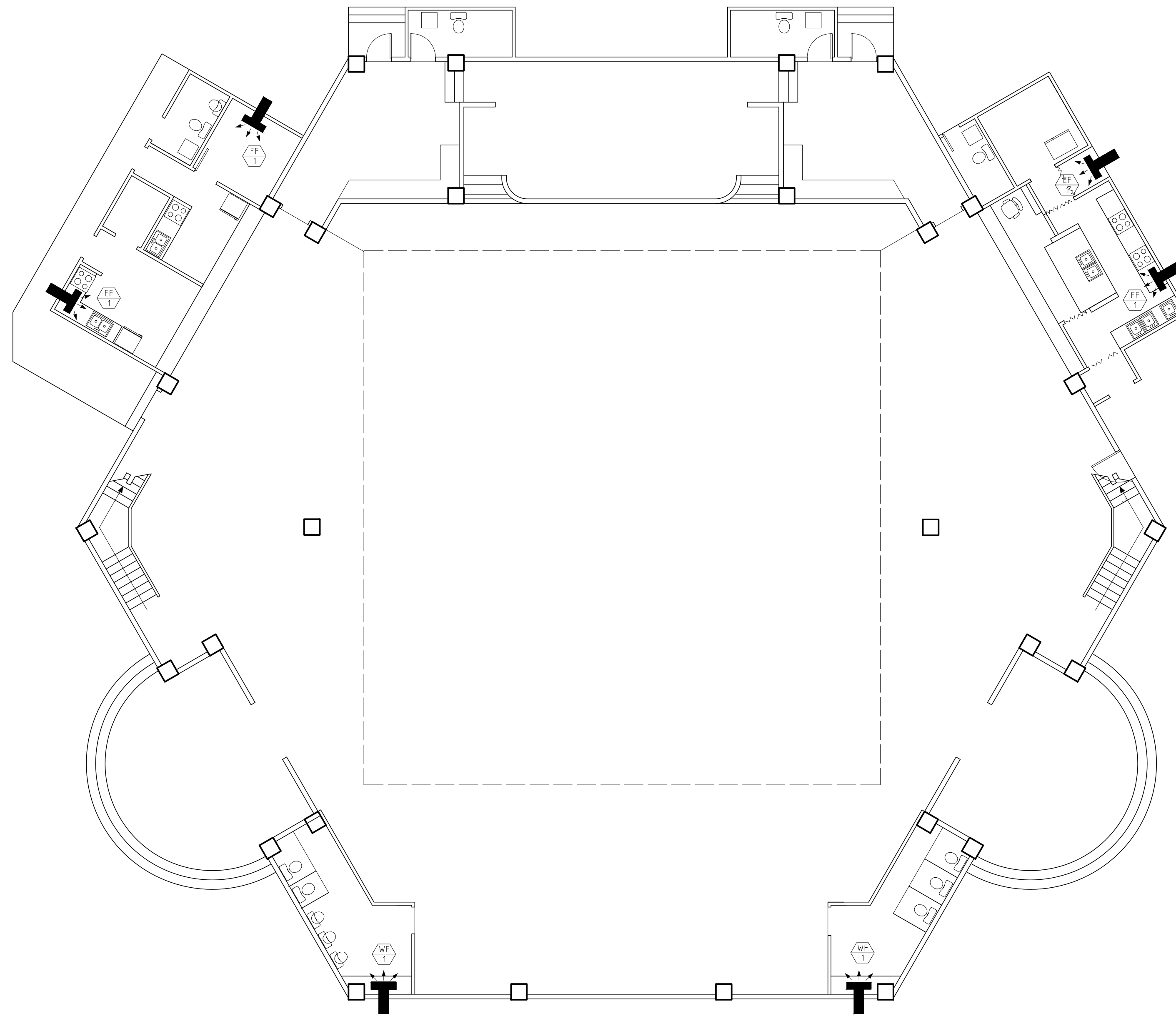
1 GROUND FLOOR VENTILATION LAYOUT ML 01 SCALE 1: 100 MTS.
