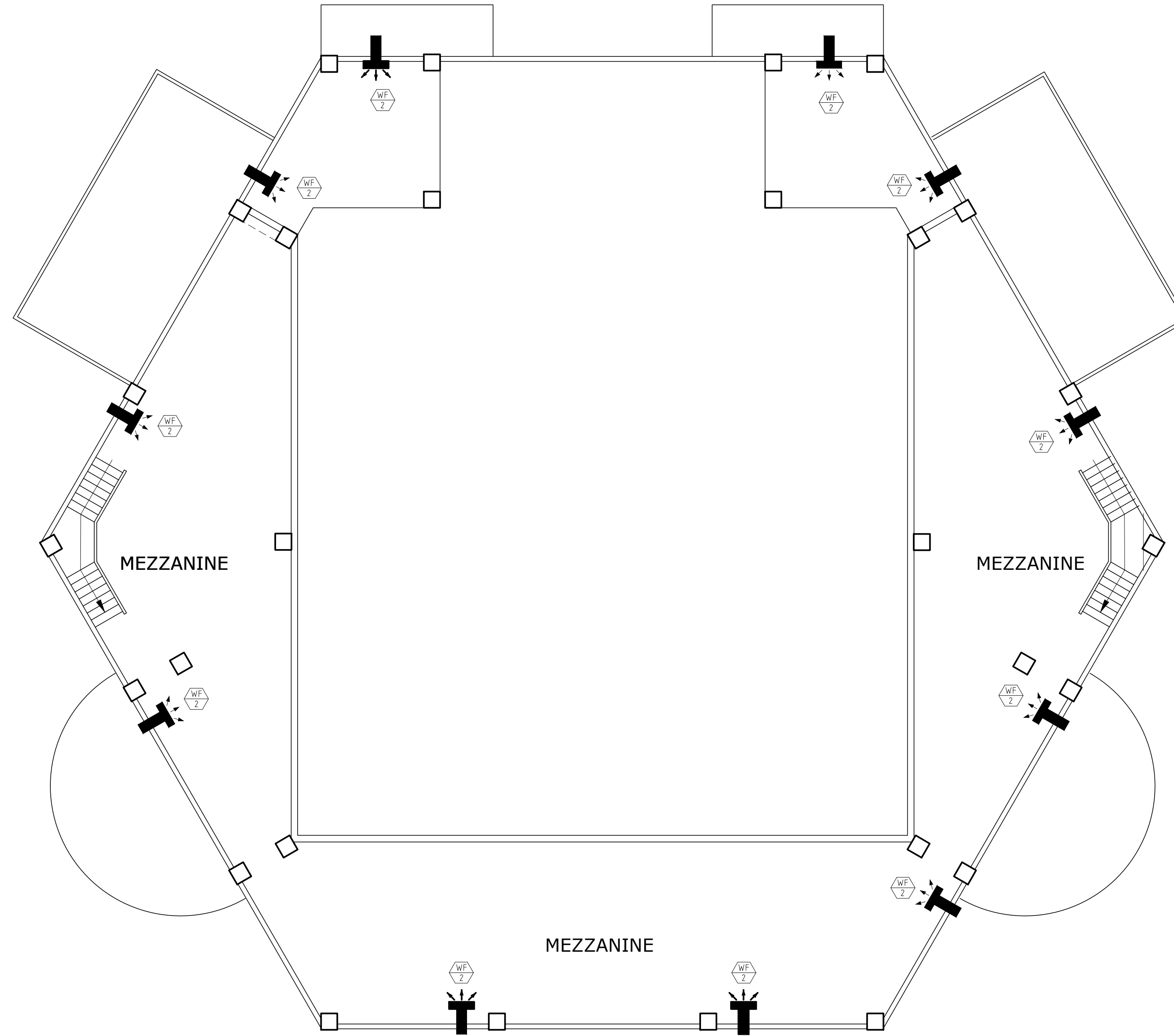
1 MEZZANINE VENTILATION LAYOUT ML 02 SCALE 1: 100 MTS.
