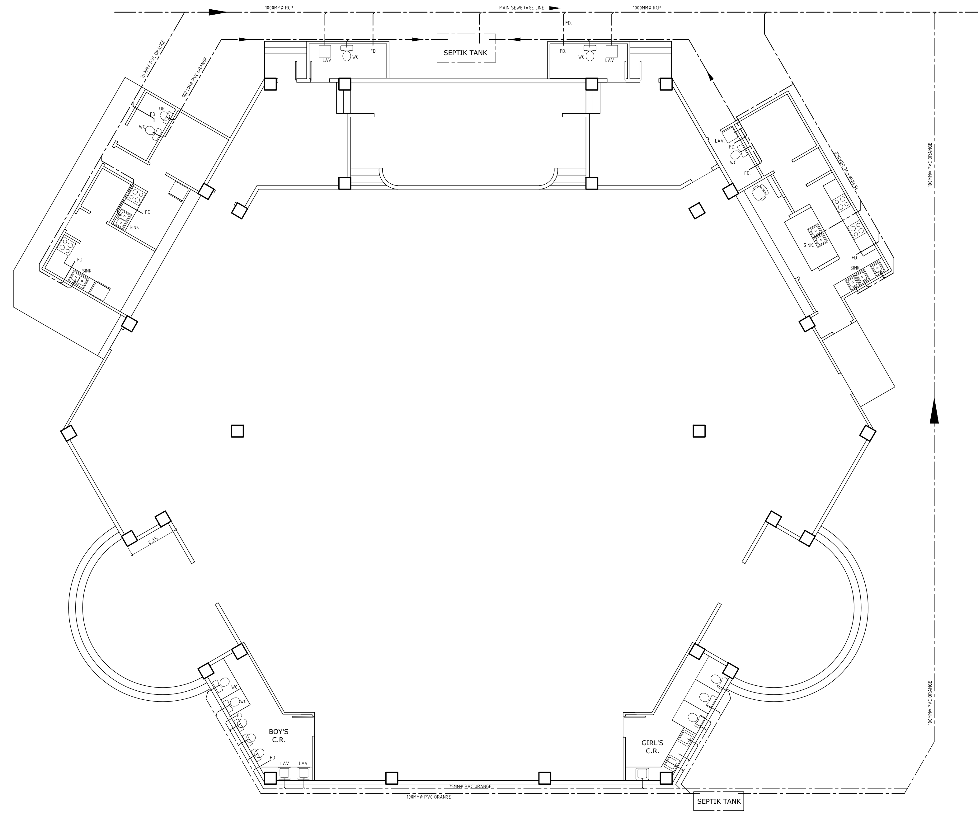
1 SEWER LINE LAYOUT PL 01 SCALE 1: 100 MTS.
