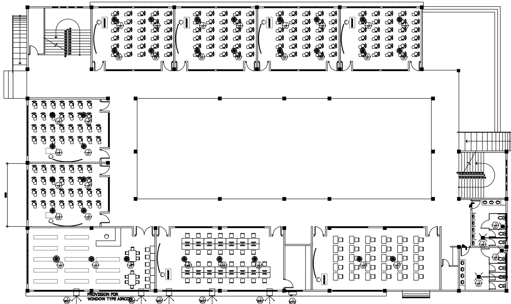
PROVISION FOR WINDOW TYPE AIRCOOL PROVISION FOR WINDOW TYPE AIRCOOL 1 M-2 SCALE 1:100M AC & VENTILATION LAYOUT
