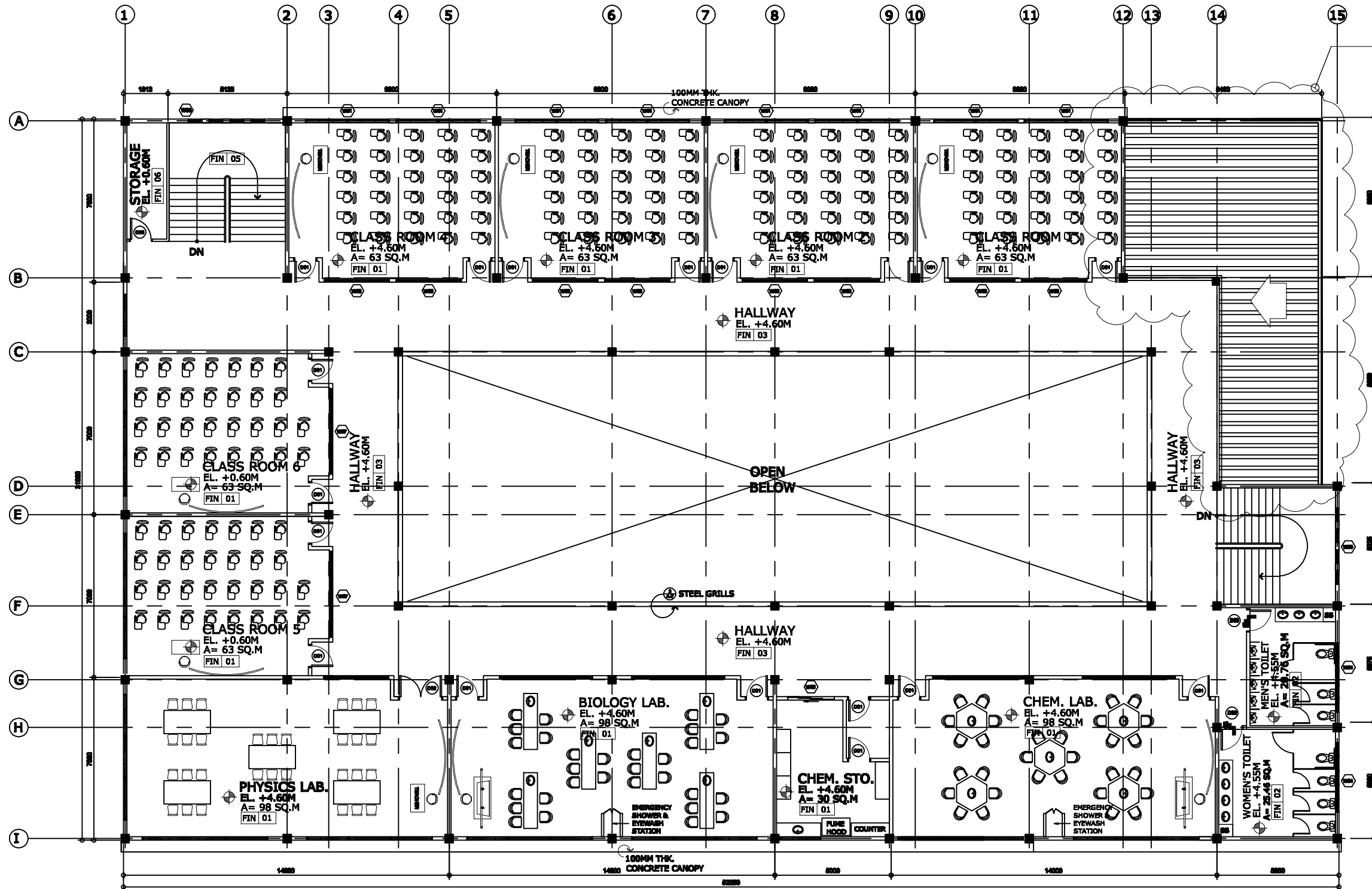
1 SECOND FLOOR PLAN A-3 SCALE 1:100M
