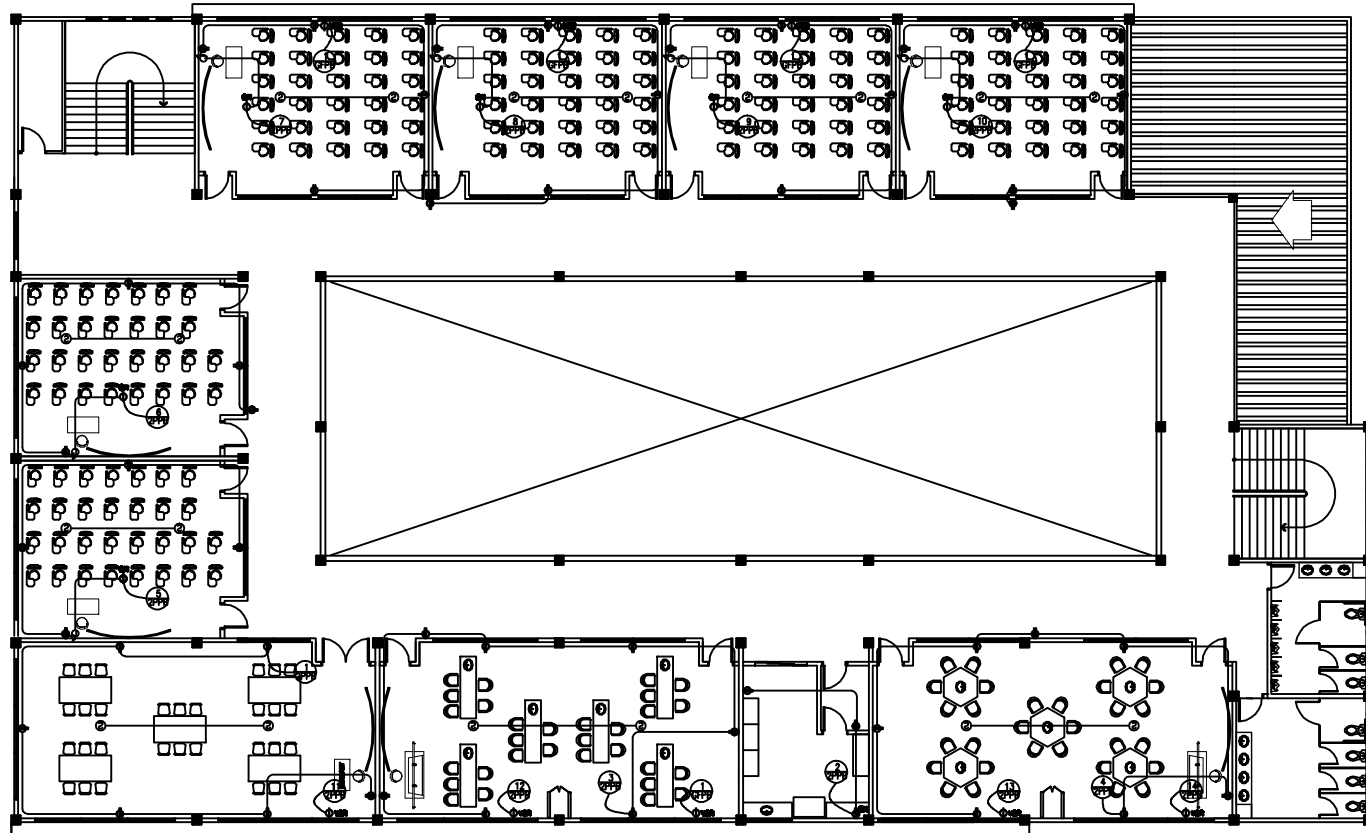
1 GROUND FLOOR POWER LAYOUT SCALE 1:100M
