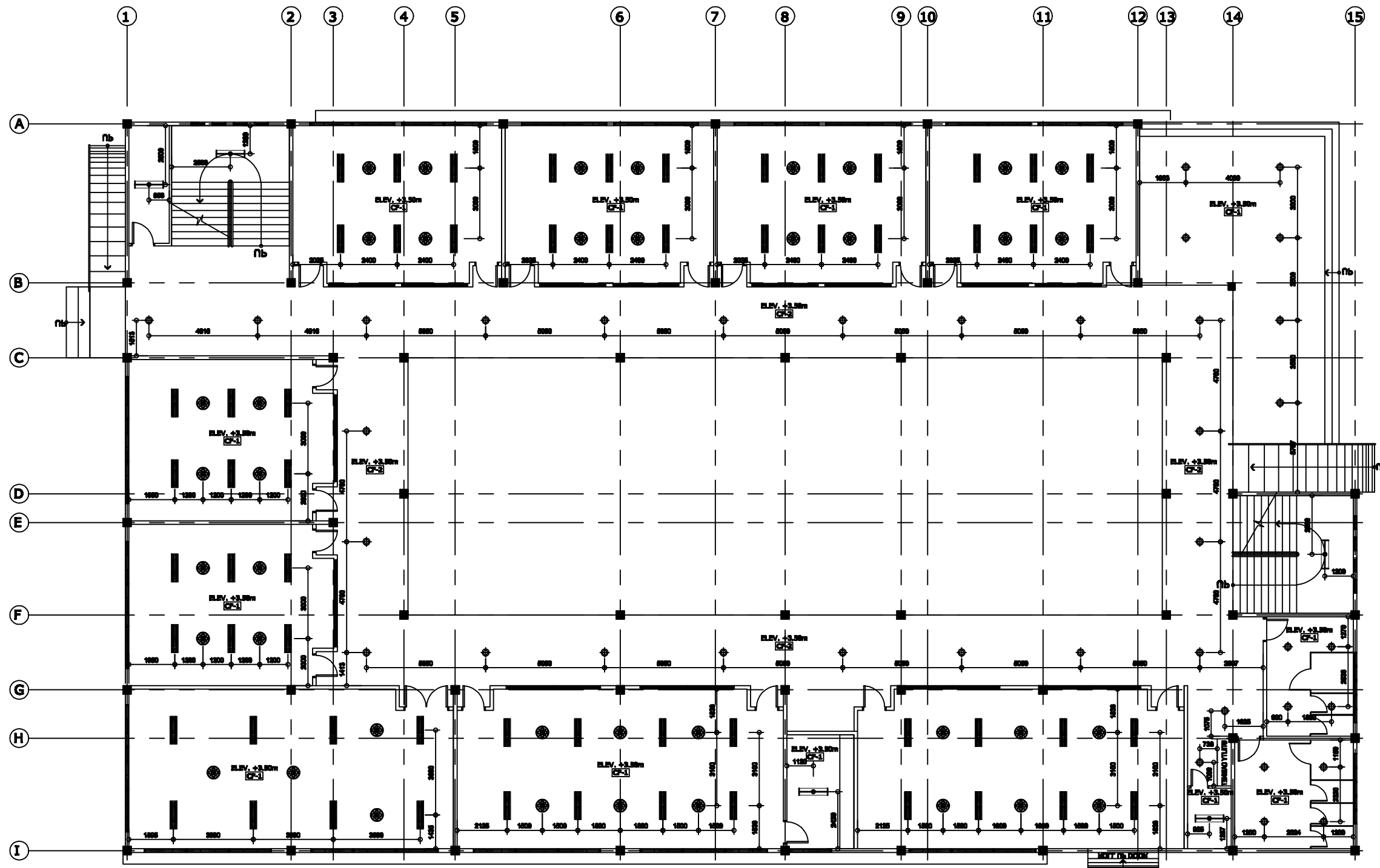
1 A-8 REFLECTED CEILING PLAN GROUND FLOOR PLAN SCALE 1:100M
