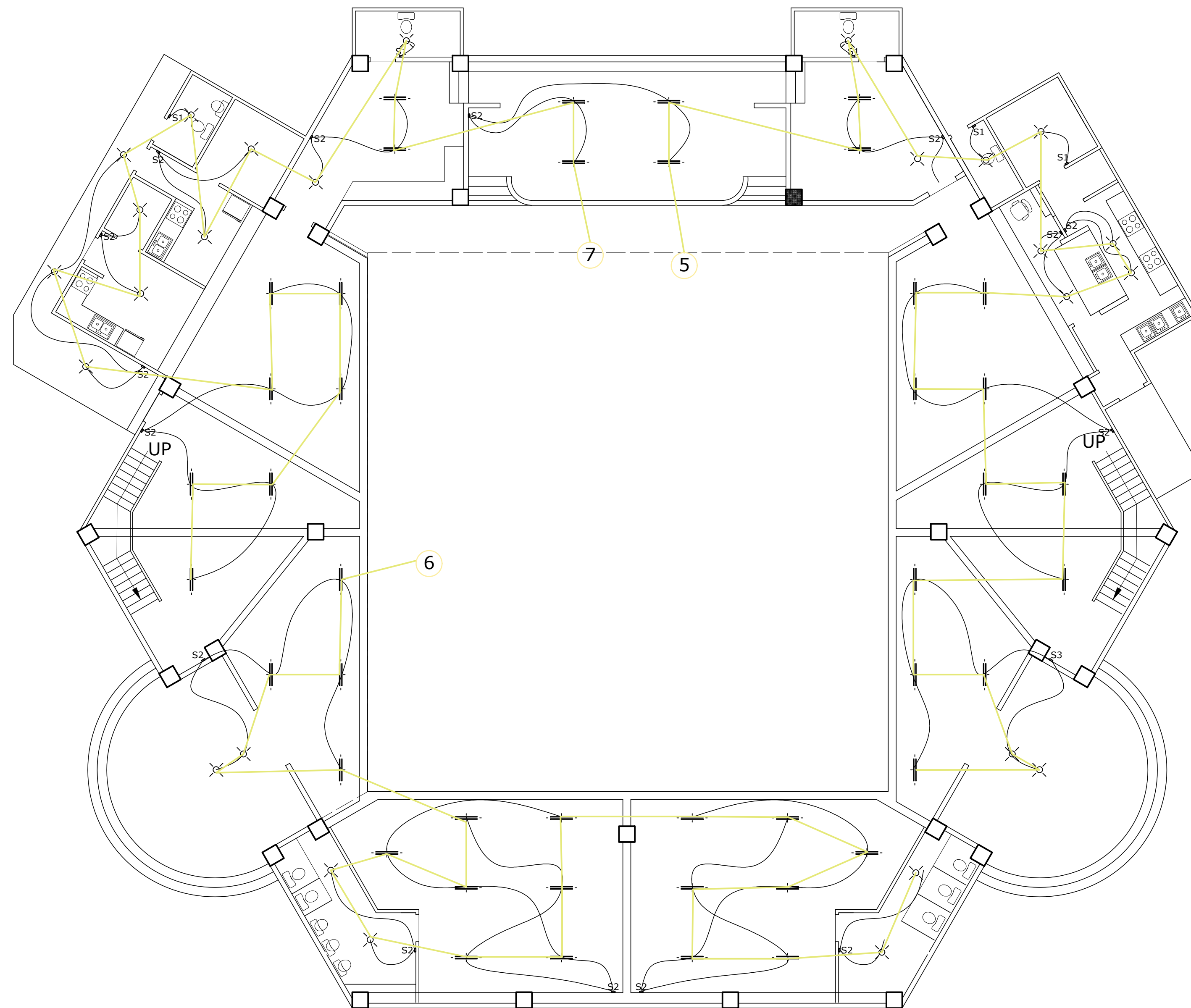
1 EL 03 GROUND FLOOR LIGHTING LAYOUT SCALE 1: 100 MTS.
