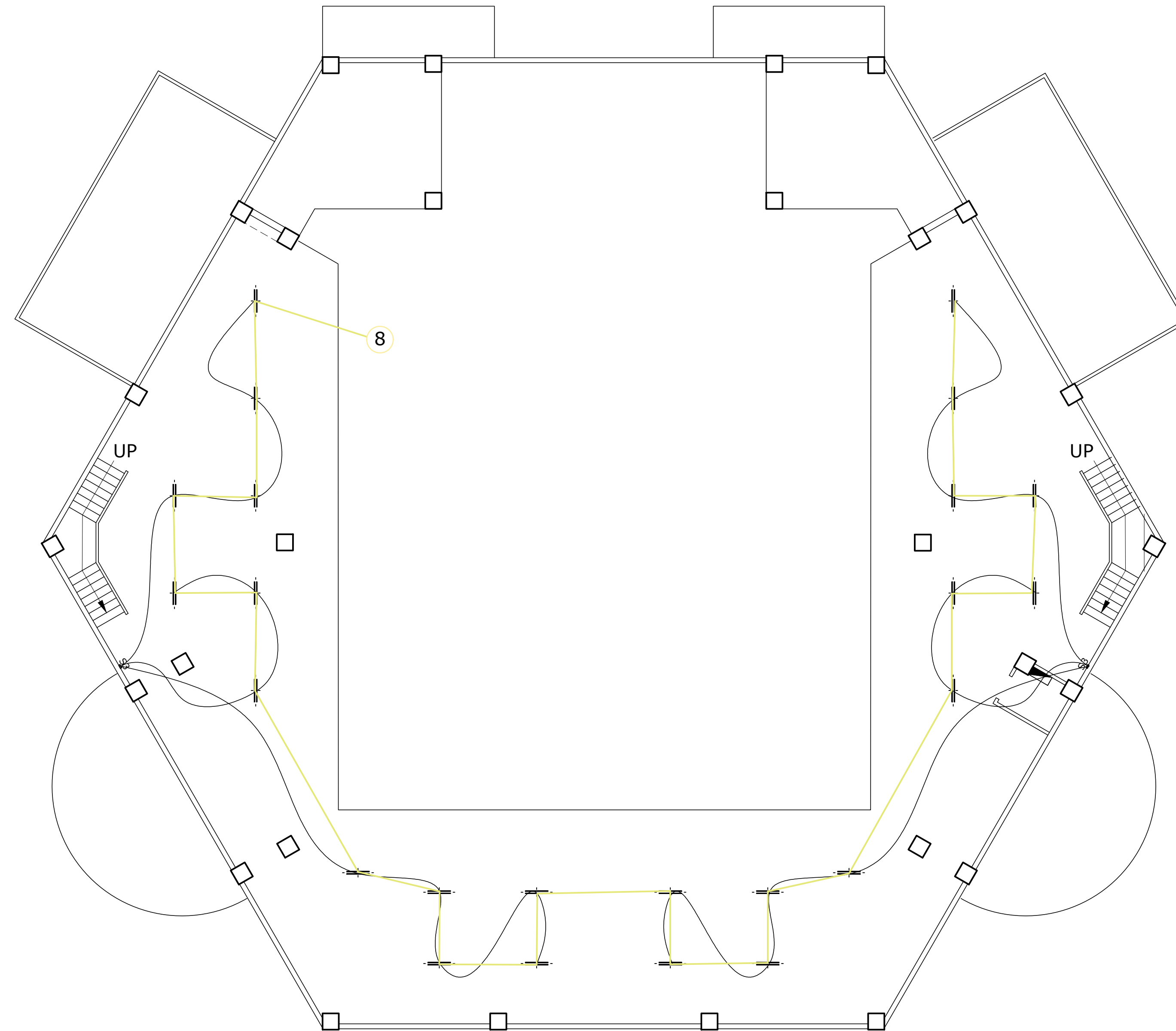
1 MEZZANINE LIGHTING LAYOUT EL 04 SCALE 1: 100 MTS.
