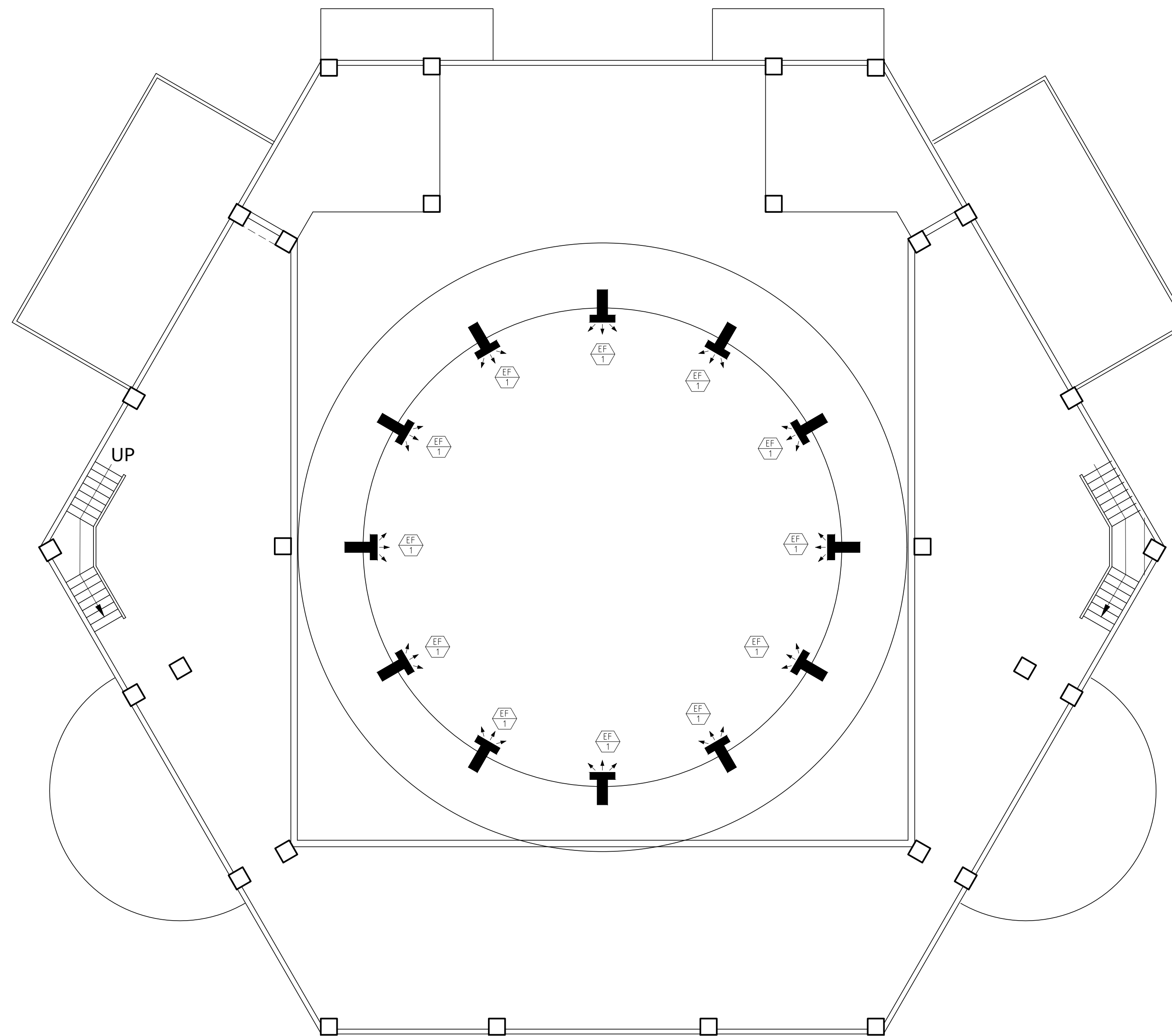
1 ROOF VENTILATION LAYOUT ML 03 SCALE 1: 100 MTS.
