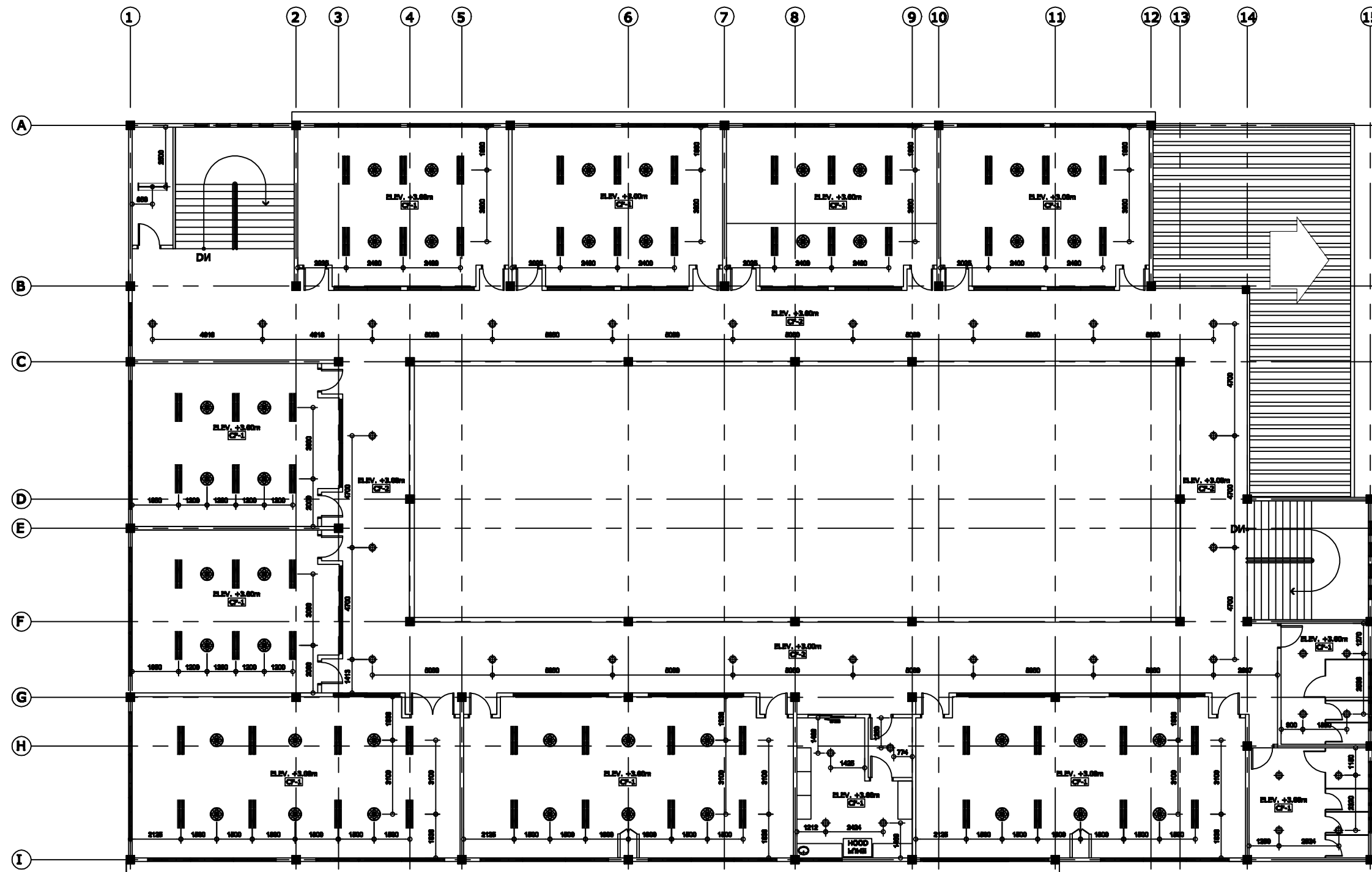
1 REFLECTED CEILING PLAN SECOND FLOOR PLAN A-9 SCALE 1:100M
