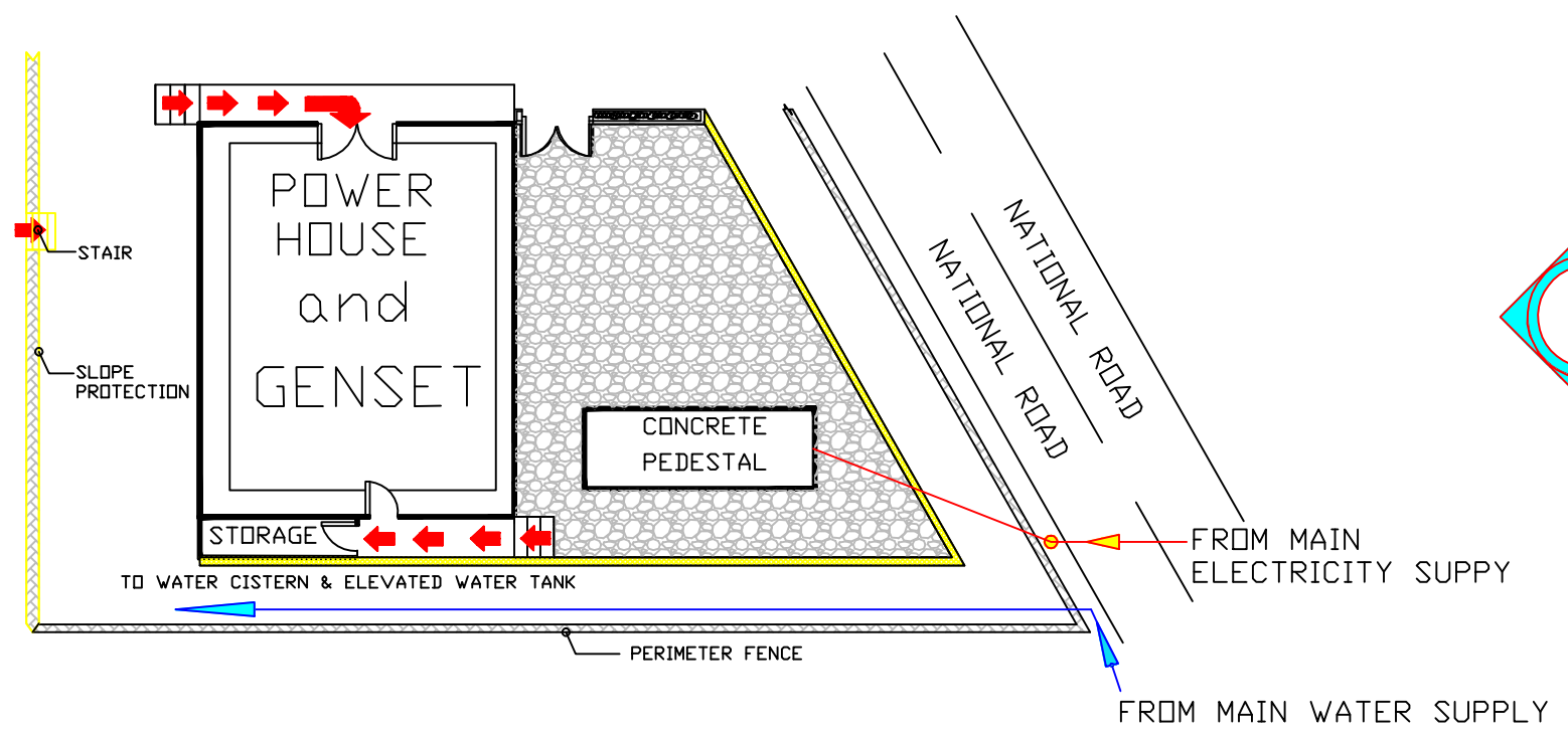
E 08 MAIN POWER HOUSE AND CONCRETE PEDESTAL LOCATION SCALE _____ NTS
